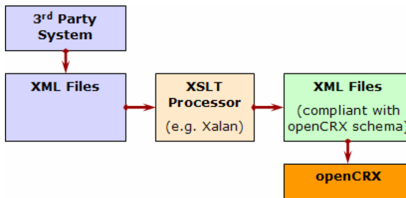
Figure 47: XML import from 3 rd party system – overview
