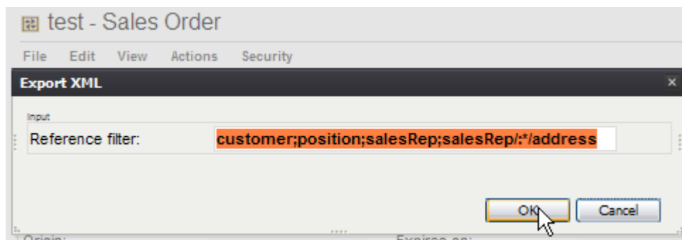
Figure 51: Exporting SalesOrder as XML File
