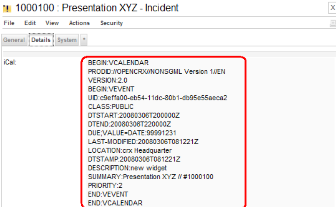
Figure 41: An openCRX activity's iCal representation
