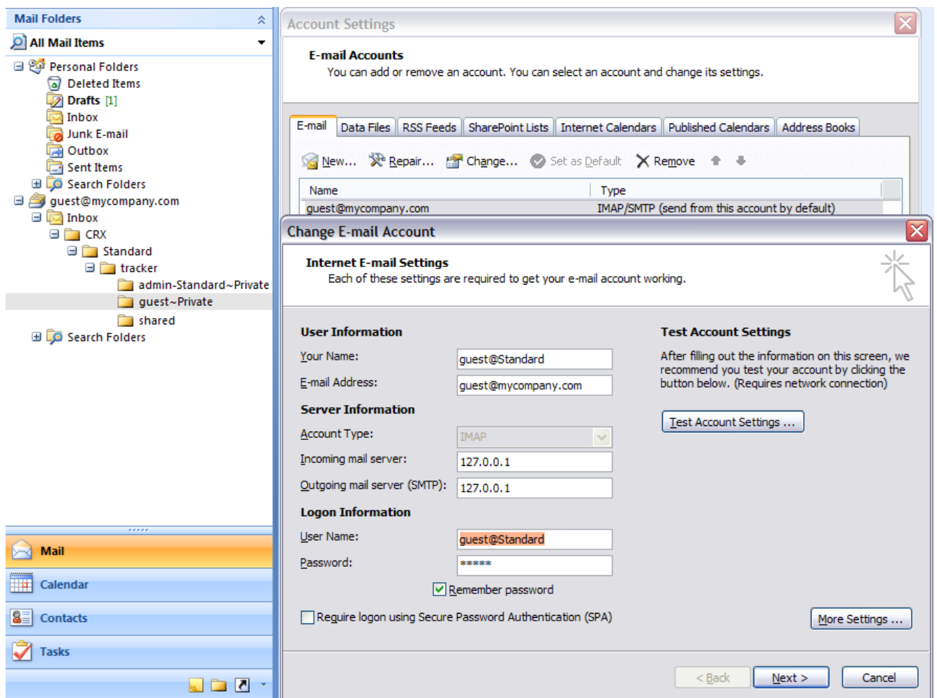
Figure 46: Thunderbird IMAP Configuration
