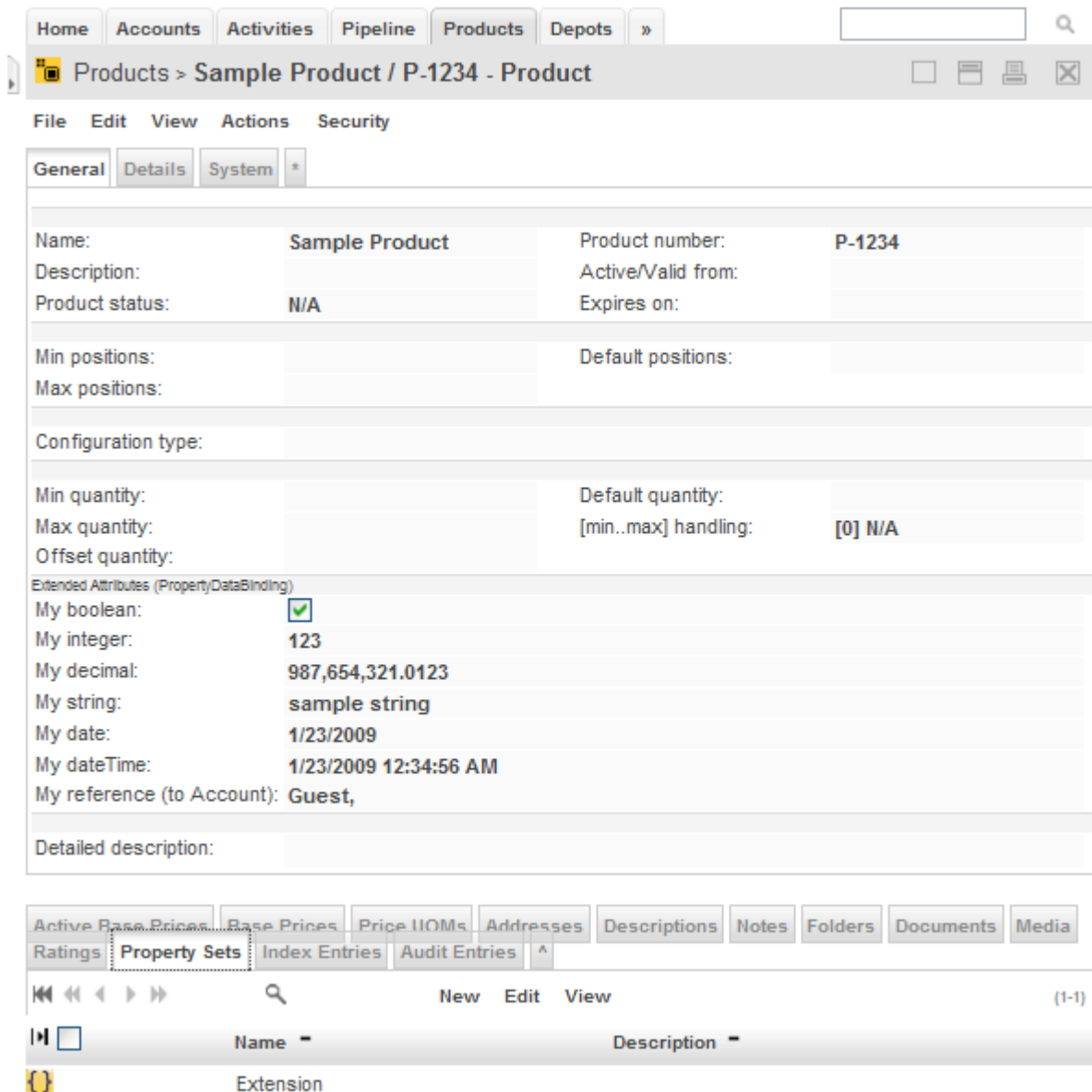
Figure 15: Sample Extension of class Product with PropertyDataBindings
